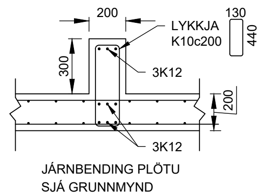
04 SNID B002 B003 B004 1:20
