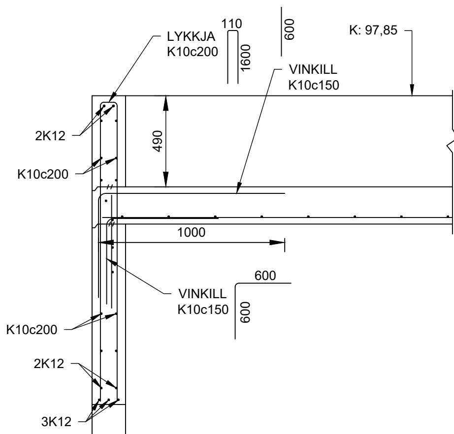
03 SNID B002 B003 B004 1:20
